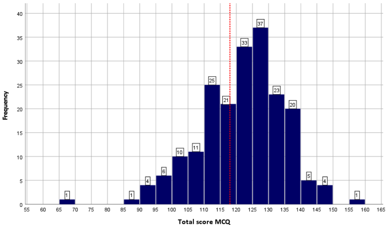
Figure 1: Distribution of scores
