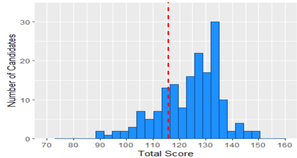
Figure 1: Distribution of scores (red dotted line denotes pass mark)
